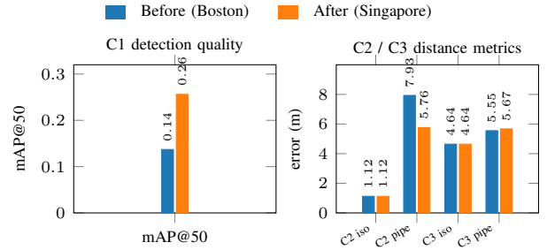
Fig. 3: Reference update on singapore_val , before versus after: (a) C1 detection quality, (b) C2/C3 distance metrics.
