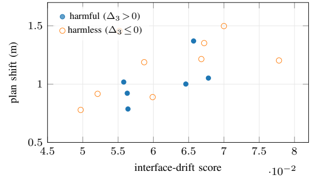
Fig. 6: Interface drift vs. plan shift over the 15 full-trainval updates (Spearman \approx 0.56 ). Drift tracks the magnitude of plan movement, but harmful and harmless updates are interleaved, so drift alone does not classify harm (AUROC \approx 0.48 ).
