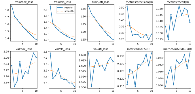
Fig. 7: YOLOv11n C_1 Boston fine-tune training curves.
